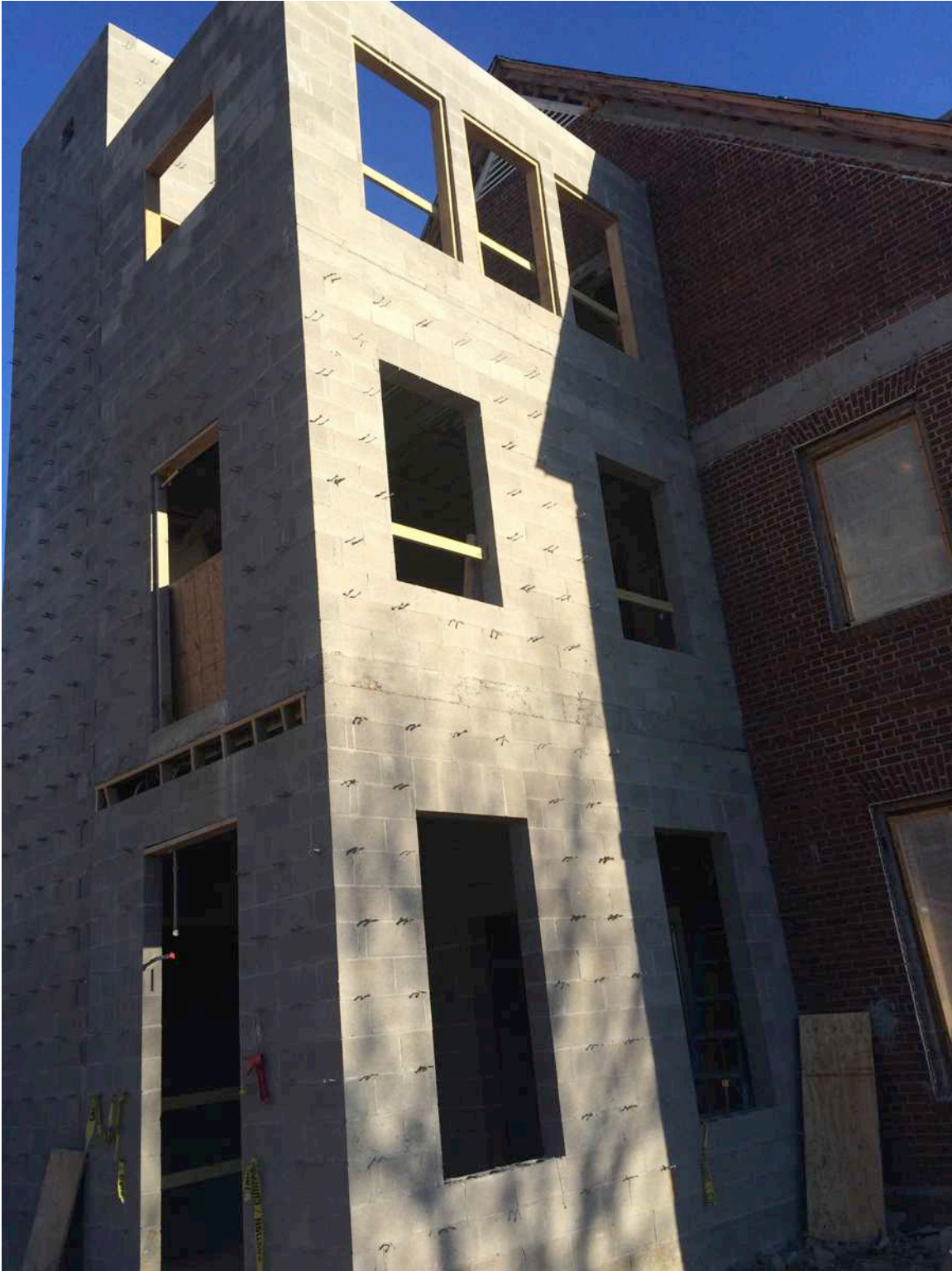
North side elevator addition.
